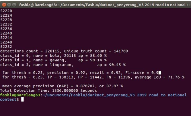
Fig. 13. Datasets Performance of YOLO v3
