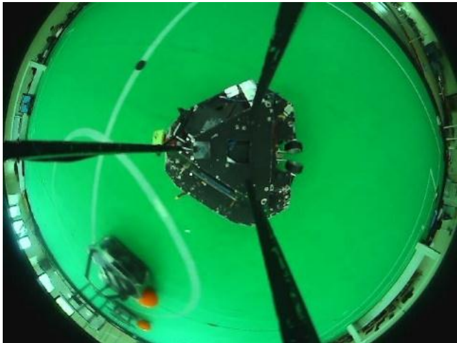
Fig. 9. Example Picture
