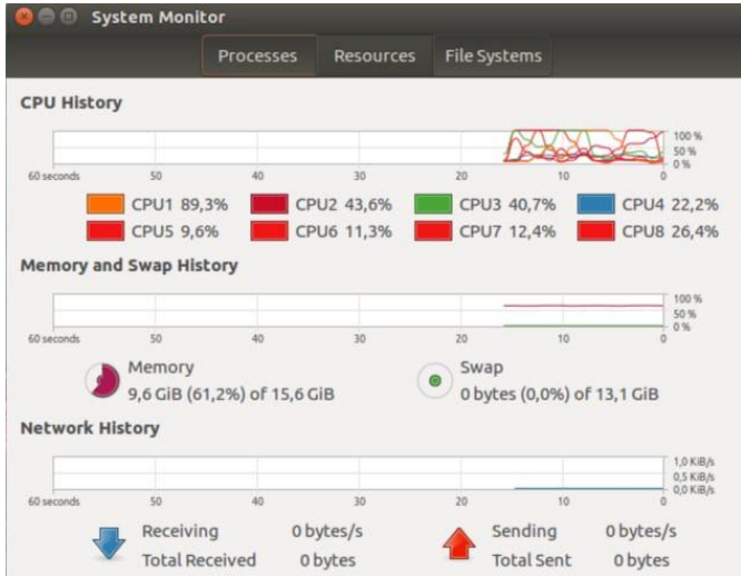
Fig. 10. Resources CPU
