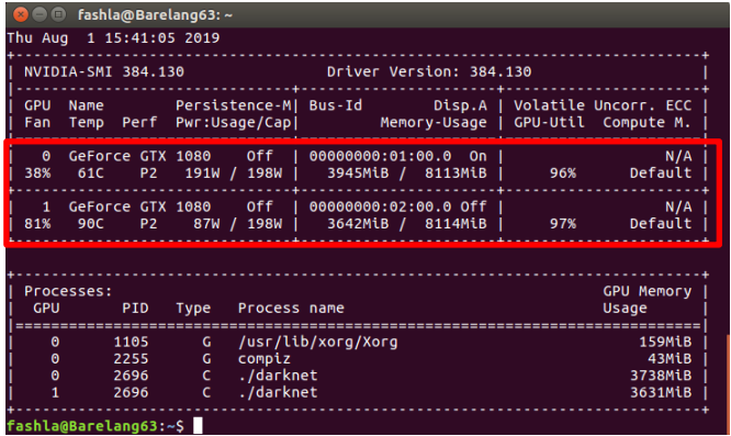
Fig. 11. Resources GPU
